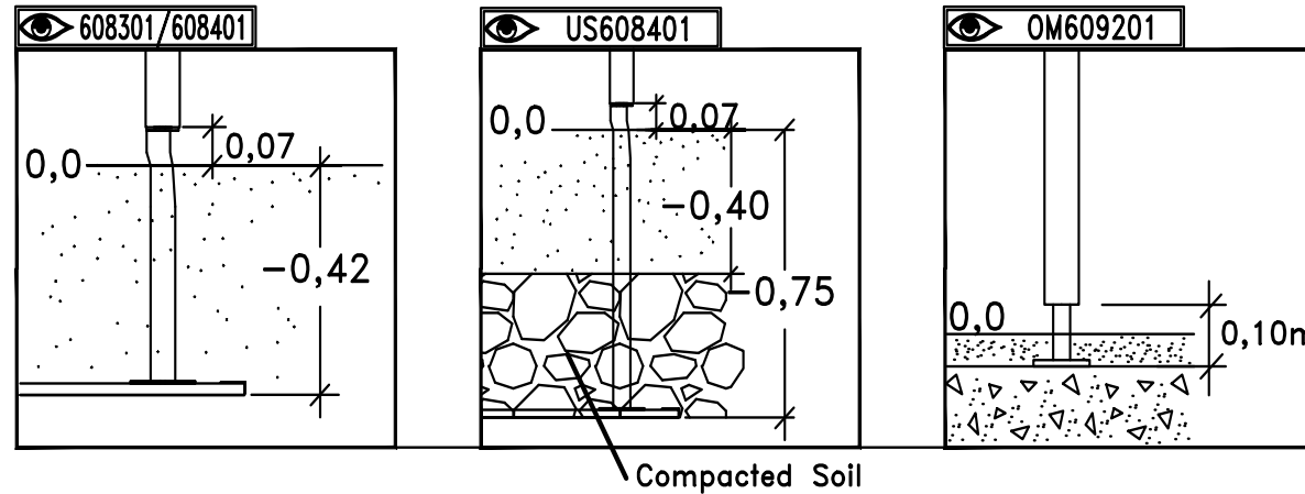
SF Sunken Foundation 8104296
