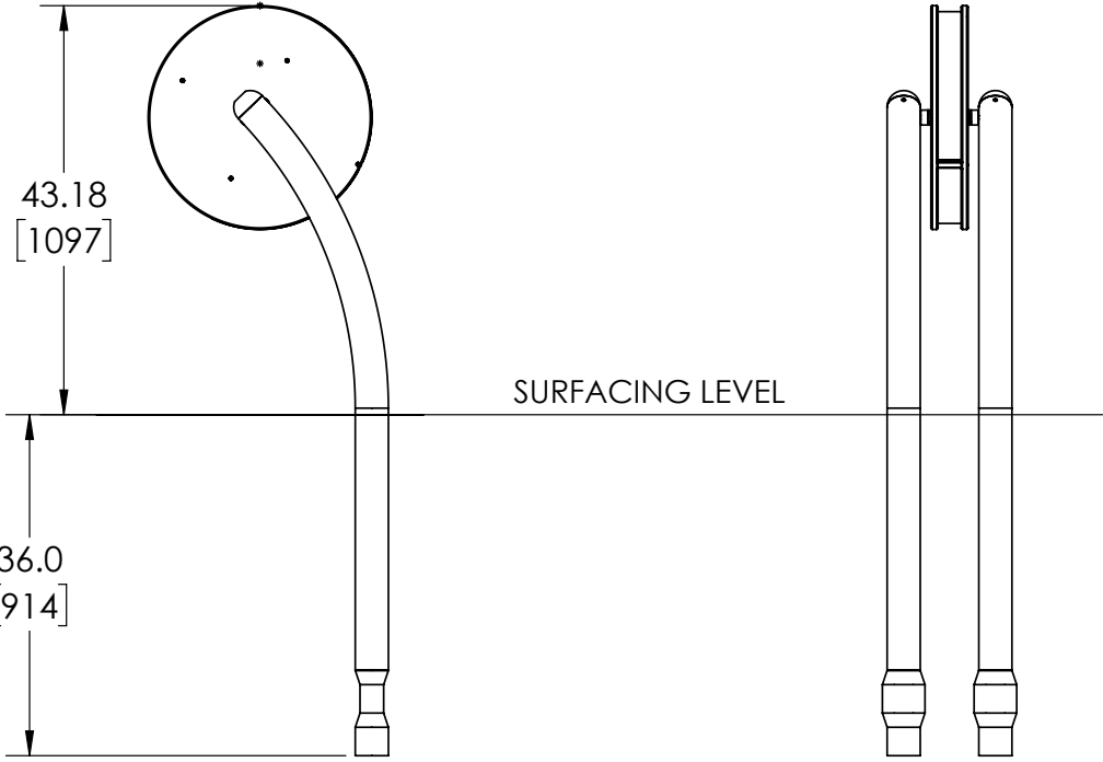
Elevation Views
